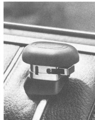
Rear-door Child Lock Guards (4-Door Models Only). Prevents children from unlocking and opening rear doors. When buttons are down and Lock Guards are pushed in, rear doors can't be opened without inserting key into lock button. 1—Unlock position. 2—Regular locked position. 3—Lock Guard position. Any of your regular car keys may be used to release the Lock Guards. (D)
