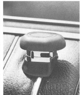
Rear-door Child Lock Guards (4-Door Models Only). Prevents children from unlocking and opening rear doors. When buttons are down and Lock Guards are pushed in, rear doors can't be opened without inserting key into lock button. 1—Unlock position. 2—Regular locked position. 3—Lock Guard position. Any of your regular car keys may be used to release the Lock Guards. (D)
